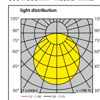
Panel LED 600 x 600mm - Neutral white
