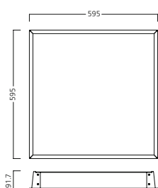
PanelLED - 600 x 600mm
