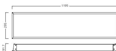
PanelLED - 1200 x 300mm
