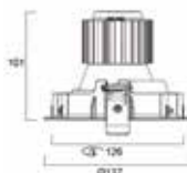
Expospot 70mm Ajustable
